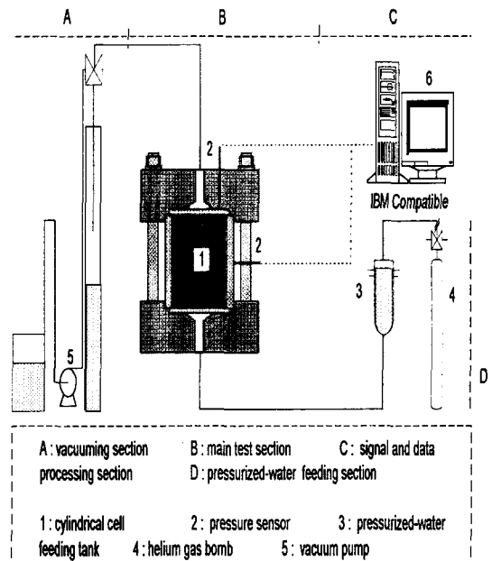
Fig. 3. Experimental Apparatus for Measuring the Swelling Pressures
