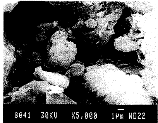
(a) dry density = 1.6Mg/m 3
