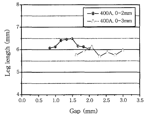
Fig. 3 Leg length measurement for test results
