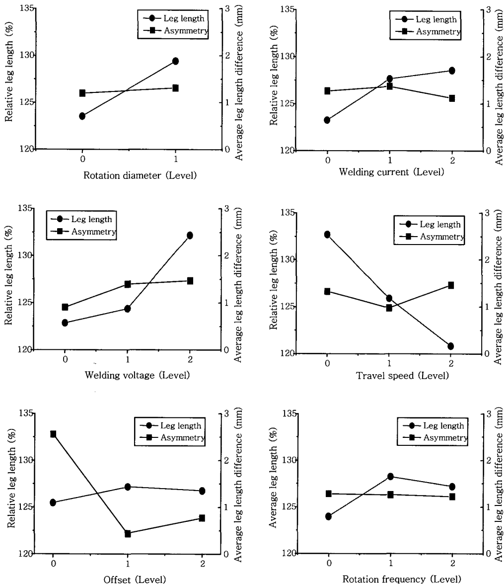
Fig. 1 Effect of welding parameters on leg length characteristics
