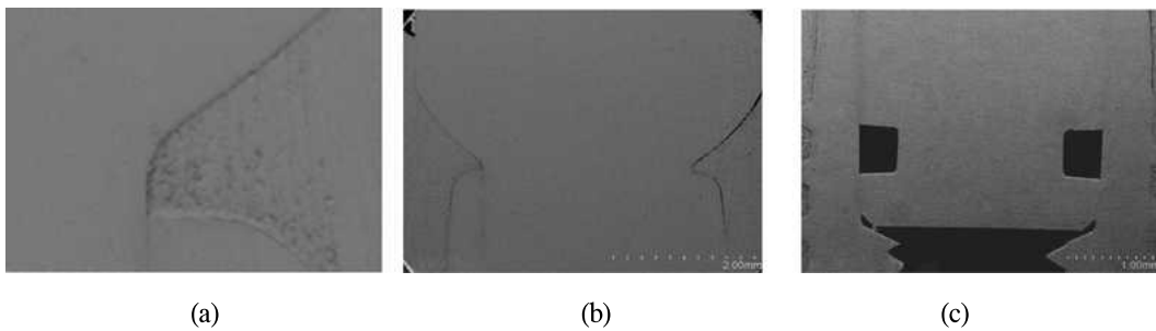
Fig. 17. FE-SEM view of Load 4 : conventional abutment. (a: x150, b: x25, c: x25)
