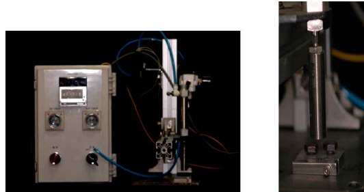
Fig. 4. Loading application instrument.
