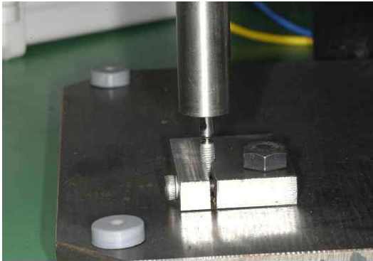
Fig. 5. Loading to abutment-fixture.
