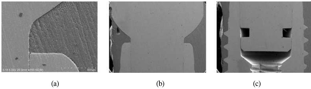
Fig. 15. FE-SEM view of Load 2 : conventional abutment. (a: x150, b: x25, c: x25)
