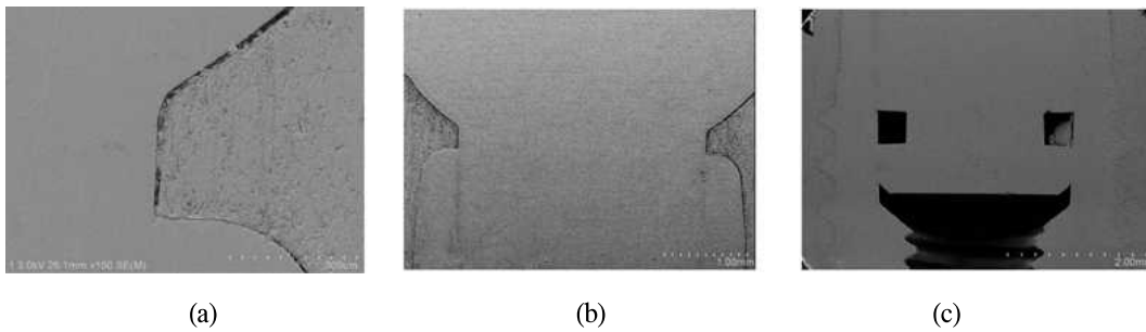
Fig. 16. FE-SEM view of Load 3 : conventional abutment. (a: x150, b: x25, c: x25)
