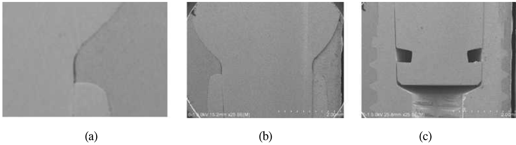
Fig. 23. FE-SEM view of Load 5 : FDI abutment. (a: x60, b: x25, c: x25)
