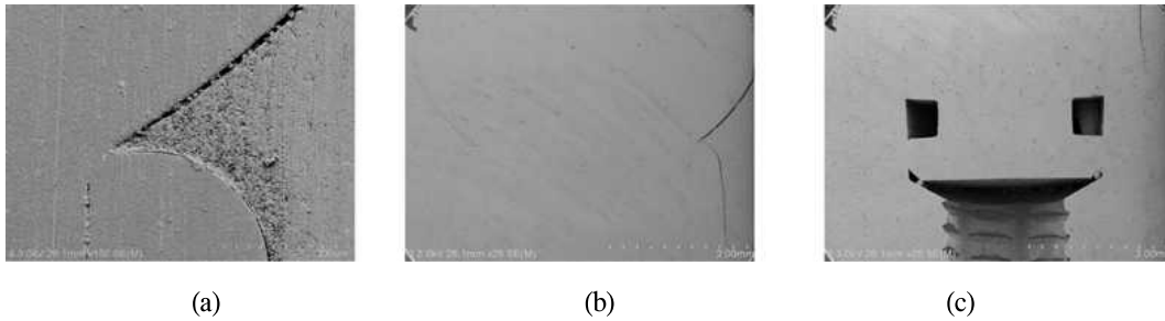
Fig. 18. FE-SEM view of Load 5 : conventional abutment. (a: x150, b: x25, c: x25)
