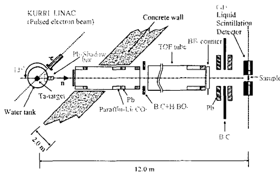
Fig 1. Experimental arrangement for the linac time-of-flight method.
