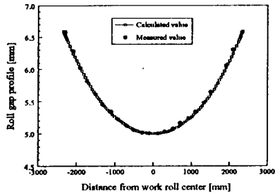
Fig.6 Comparison between calculated and measured roll gap
