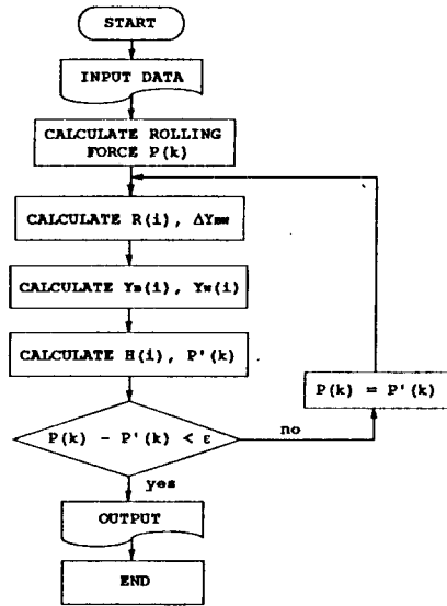
Fig.5 Flow chart for calculating plate thickness profile
