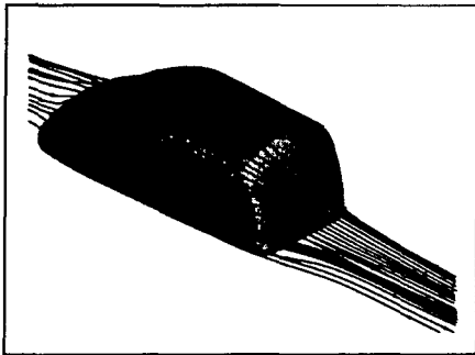
(a) 3D streamlines viewing from the oblique-back side
