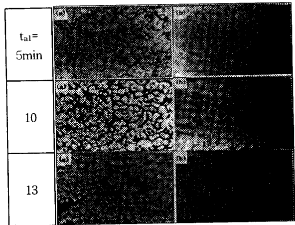
Figure 12 (a)~(b) Microstructure of ALTHIX reheated at condition of T_h=590^\circ\text{C} , t_h=2 , Q=4.97\text{kW} , specimen size= d 75 \times 60(\text{mm})
