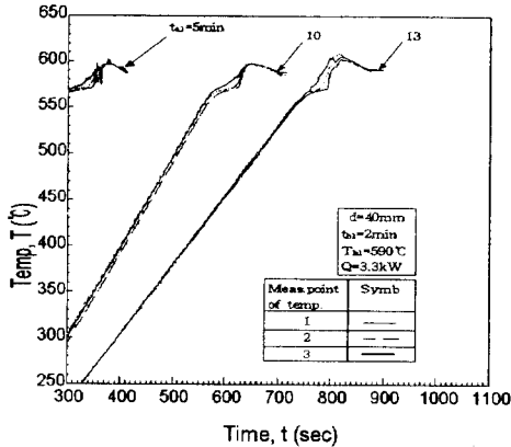
Figure 7 Relationship between reheating time and temperature to obtain globular microstructure from semi-solid aluminum alloy
