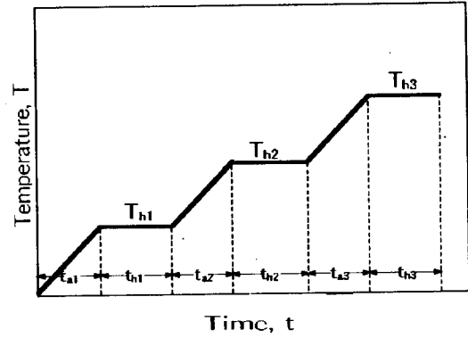
Figure 2 Schematic diagram for reheating conditions to obtain of the semi-solid material
