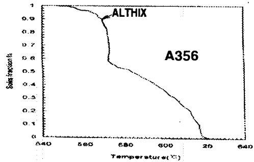
Figure 4 Relationship between solid fraction and temperature of the ALTHIX A356 aluminum alloy
