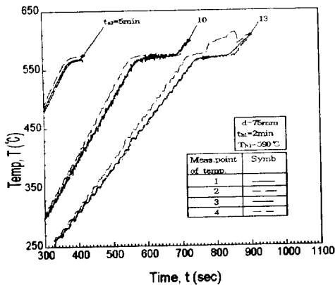
Figure 11 Relationship between reheating time and temperature to obtain the globular microstructure from semi-solid aluminum alloy in the case of experimental No 11, 12 and 13
