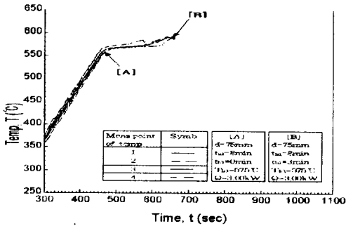
Figure 13 Relationship between holding time and temperature to obtain the globular microstructure from semi-solid aluminum alloy
