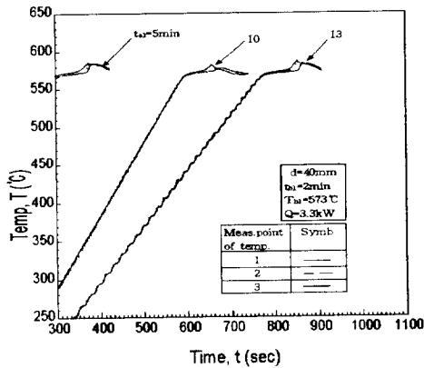
Figure 5 Relationship between reheating time and temperature to obtain globular microstructure from semi-solid aluminum alloy
