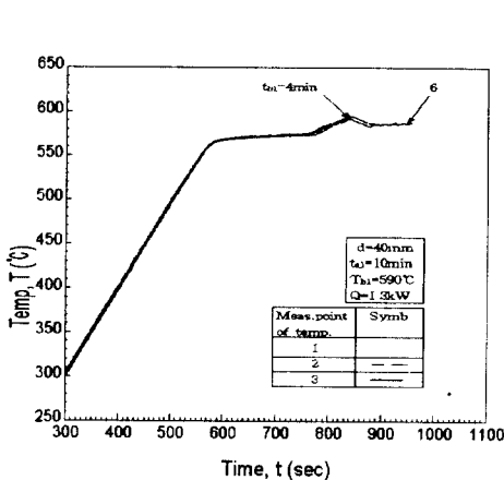
Figure 9 Relationship between reheating time and temperature to obtain the globular microstructure from semi-solid aluminum alloy
