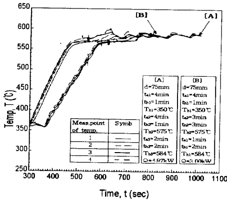
Figure 19 Temperature distributions of three steps reheating process of semi-solid alloy in condition of exp. No. 17 and 18 of Table. 1
