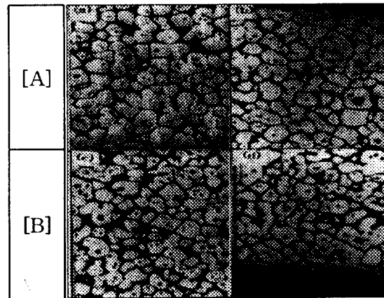
Figure 18 Microstructure in two steps reheating process of semi-solid alloy
