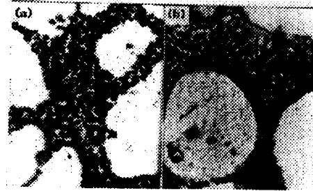
Figure 16 (a)~(b) Eutectic Microstructure of ALTHIX reheated at condition of experiment No 12 and experiment No 13
