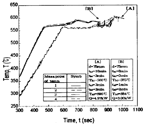
Figure 17 Temperature distributions in two steps reheating process of semi-solid alloy
