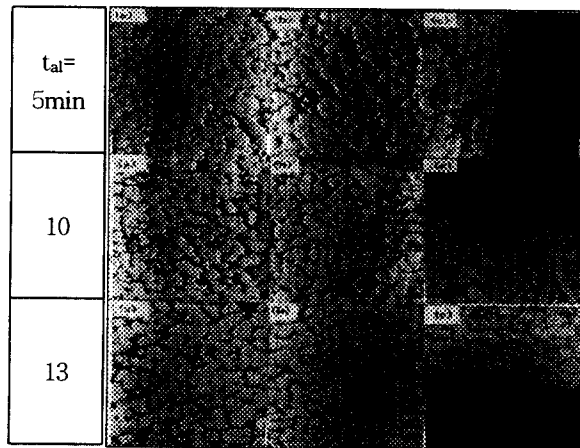
Figure 10 relationship between reheating time and temperature to obtain the globular microstructure from semi-solid aluminum alloy
