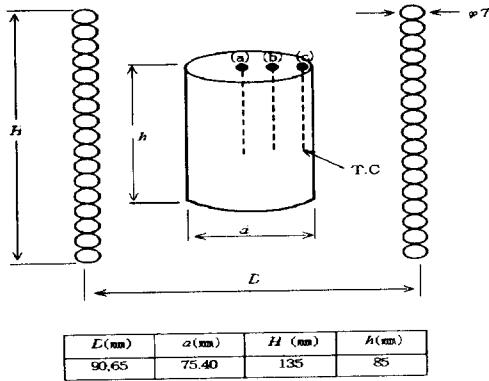
Figure 1 Schematic diagram of induction heating of cylindrical specimen
