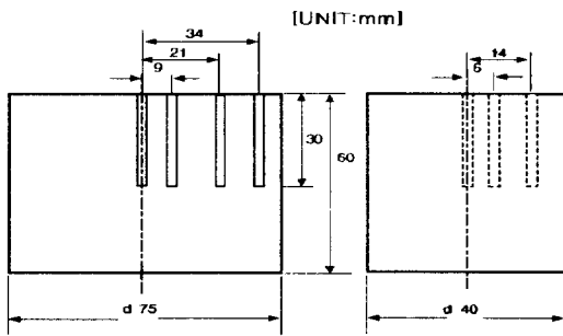
Figure 3 Schematic diagram of reheating conditions to obtain the semi-solid material
