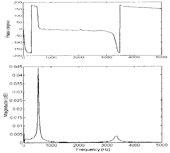
Fig. 8 Bode diagram of FRF of exciter A with stinger up to 5000Hz
