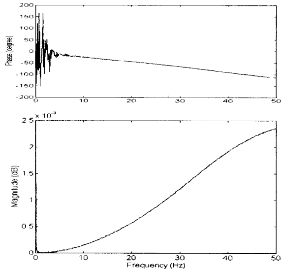
Fig. 4 Bode diagram of FRF of exciter A with bare table up to 50 Hz
