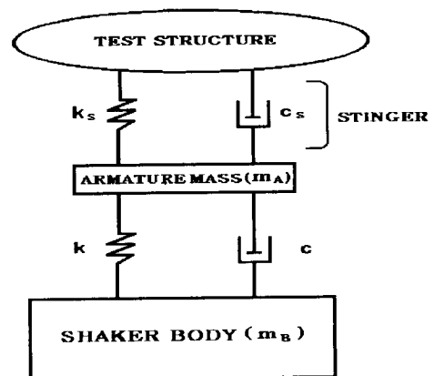
Fig. 3 Dynamic model of exciter connected to the test structure through a stinger
