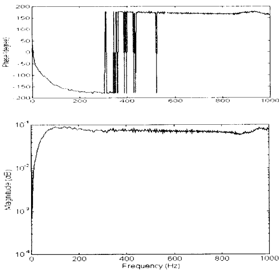
Fig. 7 Bode diagram of FRF of exciter B with bare table up to 1000Hz
