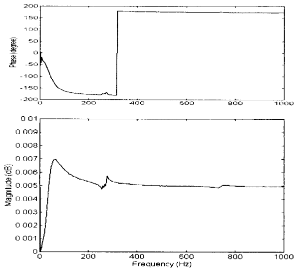
Fig. 5 Bode diagram of FRF of exciter A with bare table up to 1000Hz
