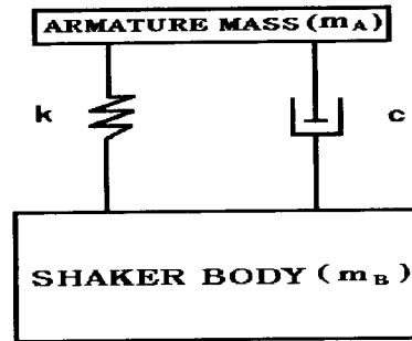
Fig. 2 Two degree of freedom model of exciter
