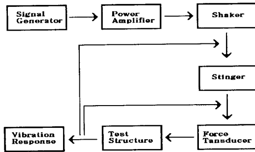
Fig. 1 Schematics of measurement for modal analysis
