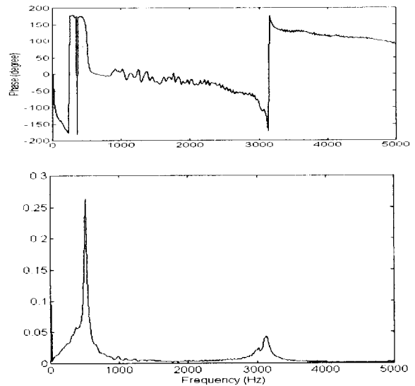
Fig. 9 Bode diagram of FRF of exciter B with stinger up to 5000Hz
