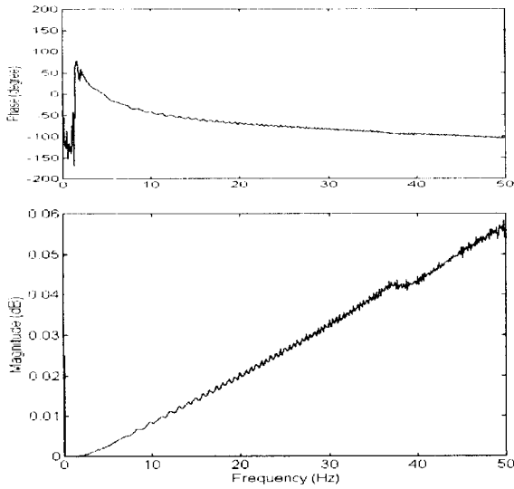
Fig. 6 Bode diagram of FRF of exciter B with bare table up to 50Hz
