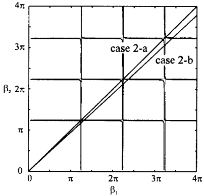
Figure 5. Characteristic graph of the case 2; case 2-a: \alpha = 1.0 ; case 2-b: \alpha = 0.95 .
