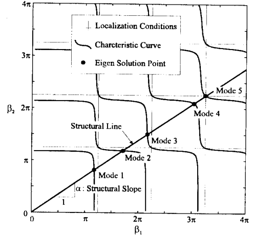
Figure 2. Characteristic graph of the two-span beam.
