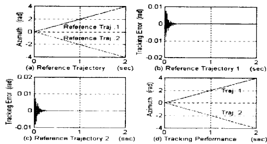
Fig.9 Control performance of the NF controller for the variation of the azimuth trajectory with parameter uncertainties (25%).
