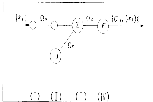
Fig.4 Neural network for gaussian membership function.
