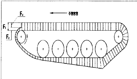
Fig. 3 Track tension of FFD vehicle.
