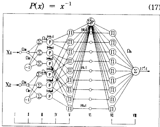
Fig.5 Basic structure of neural-fuzzy network.
