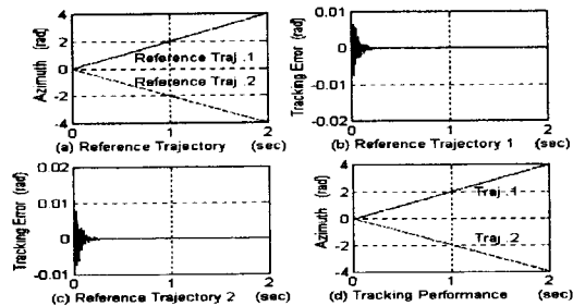
Fig.8 Control performance of the NF controller for the variation of the azimuth trajectory with parameter uncertainties (15%).
