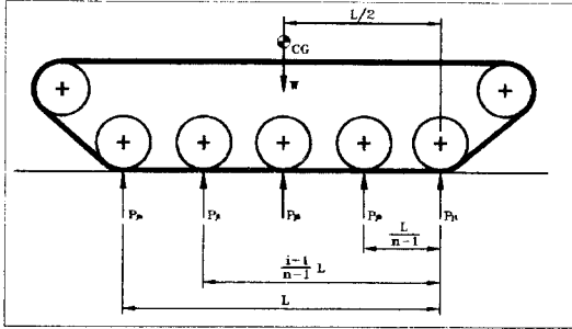
Fig.2 Load distribution of static condition.
