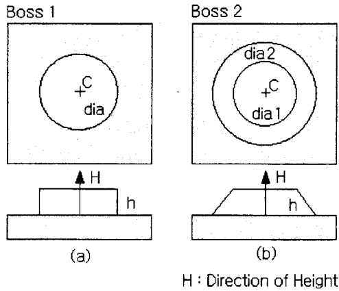
Fig. 3 A boss type feature model (a) General Boss (b) Tapered Boss
