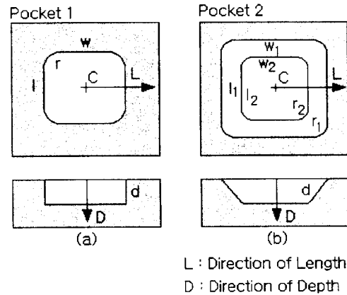
Fig. 2 A Square type feature model (a) General pocket (b) Tapered Pocket
