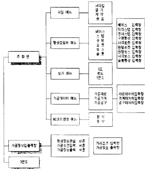
Fig. 6 The constitution diagram of user interface
