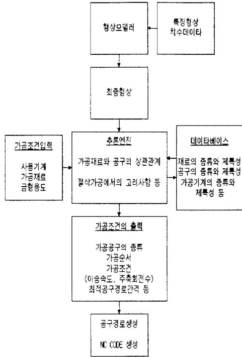
Fig. 5 Structure of Knowledge-based CAM system
