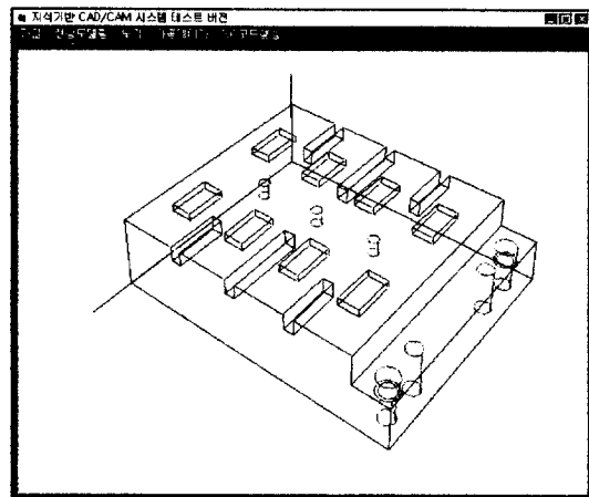
Fig. 10 Geometric model of tile type IC mold
