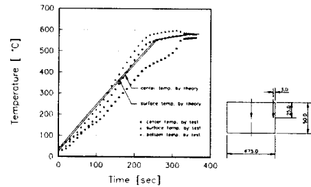
Fig.5 Variation of temperature on the heating time for measurement of temperature in induction heating apparatus
