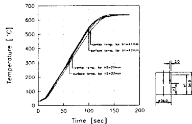
Fig.3 Variation of temperature on the heating time at different height in vertical direction
