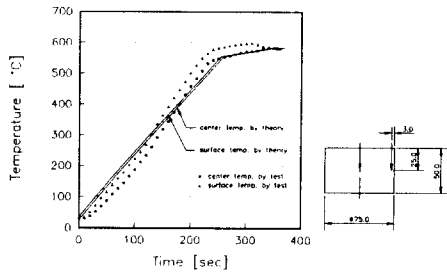
(b) 4.77 kW output
