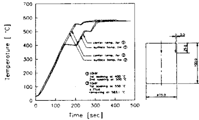
Fig.6 Variation of temperature on the heating time for step heating
