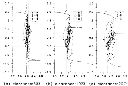
Fig. 4 Effective strain distribution.
