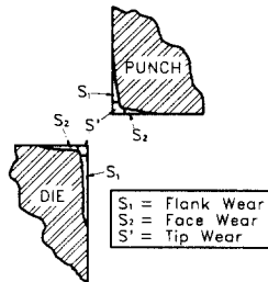
Fig. 1 Types of tool wear in sheet metal shearing.
