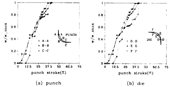
Fig. 8 Normalized wear depth of tool.(clearance: 5%)
