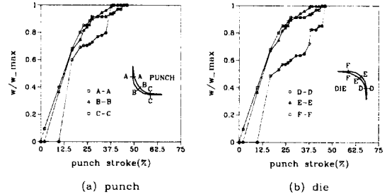
Fig. 9 Normalized wear depth of tool.(clearance : 10%)
