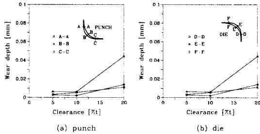
Fig. 7 Wear depth of tool with various clearances.
