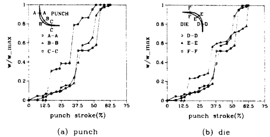
Fig. 10 Normalized wear depth of tool.(clearance : 20%)
