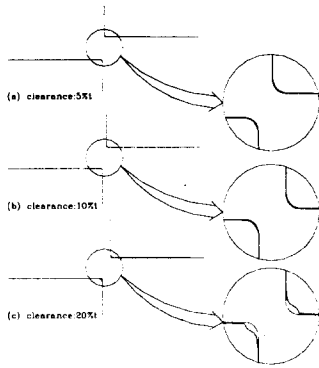
Fig. 11 Wear profiles of tool.
