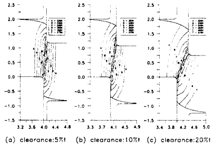
Fig. 5 Temperature distribution.
