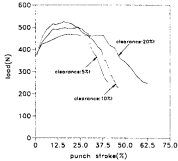
Fig. 6 Load-punch stroke diagram.
