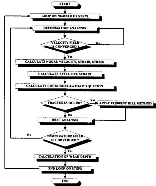
Fig. 2 Flow chart to analyze shearing process and tool wear.
