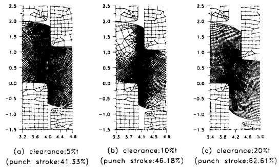
Fig. 3 Deformed mesh at final stage. (Hatched elements refer killed element)
