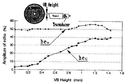
Fig.9 Relations of tool wear and amplitude of echo for artificially worn by grinding
