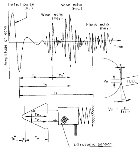
Fig.1 Wave form of tool's echo
