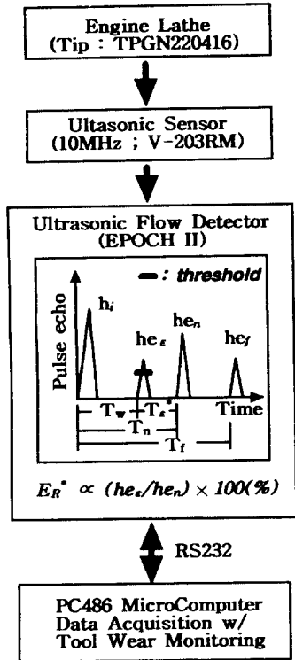
Fig.13 Configuration of the proposed tool wear monitoring system by ultrasonic method
