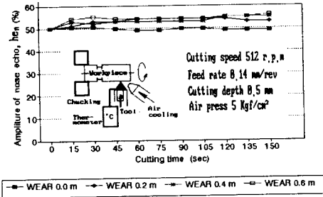
Fig.6 Relationships between cutting time and amplitude of nose echo (with air jet cooling cut)
