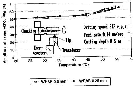
Fig.5 Temperature vs amplitude of nose echo (without air jet cooling cut)
