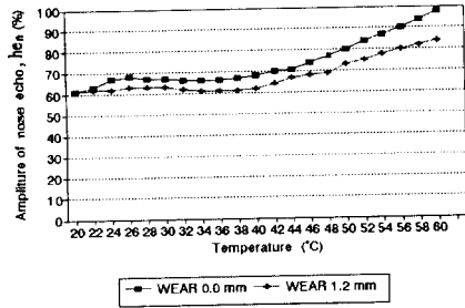
Fig.4 Temperature vs amplitude of nose echo
