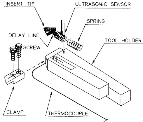
Fig.3 Tool holder and transducer assembly
