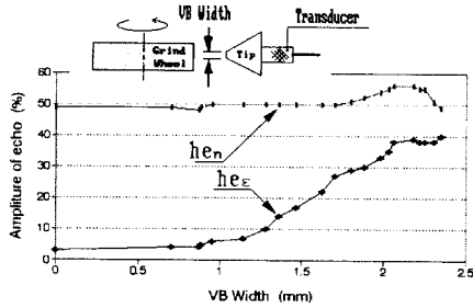
Fig.8 Relations of tool wear and amplitude of echo for artificially worn by grinding
