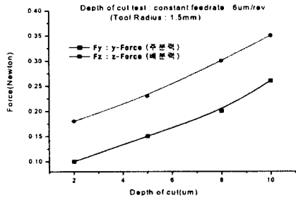
(c) Aluminum, Tool nose radius=1.5mm
