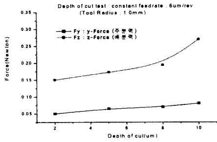
(b) Aluminum, Tool nose radius=1.0mm
