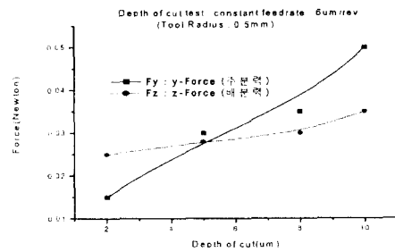
(a) Aluminum, Tool nose radius=0.5mm
