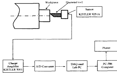
Fig. 1 Experimental setup
