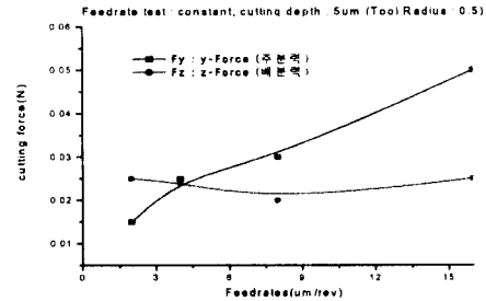
(a) Aluminum, Tool nose radius=0.5mm
