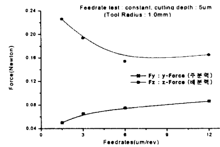
(b) Aluminum, Tool nose radius=1.0mm
