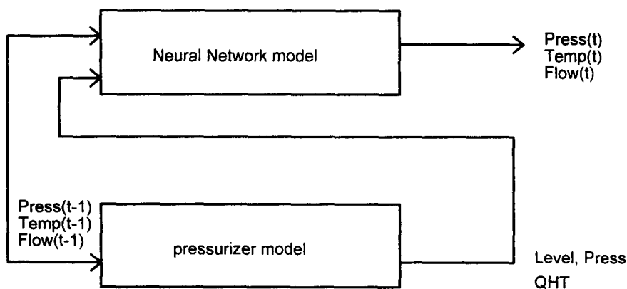
Fig. 1 Dynamic system predictor structure
