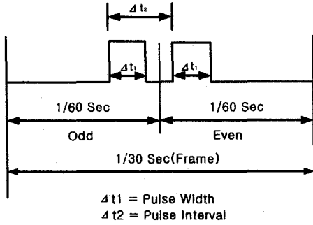
Fig.3 Video Signal and Pulse Arrangement
