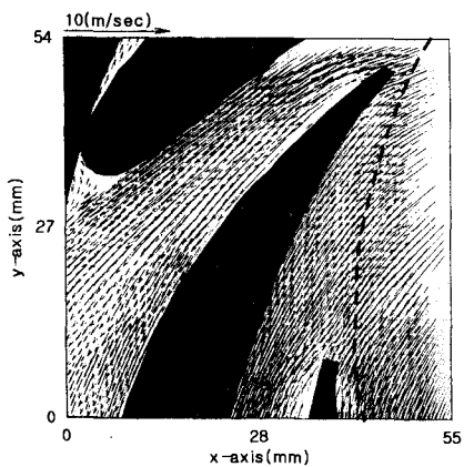
(a) Velocity Vectors
