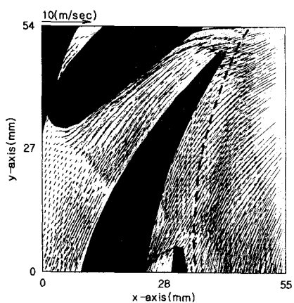
(a) Velocity Vectors
