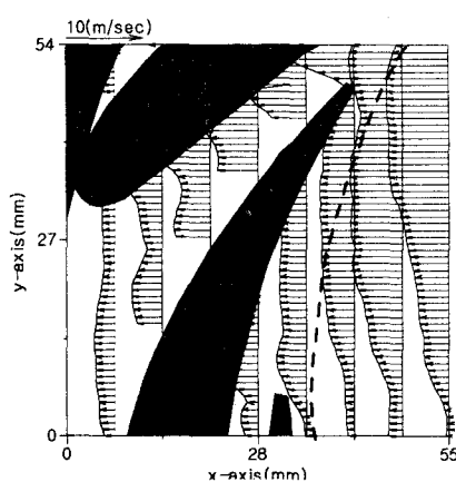
(b) Velocity Profiles
