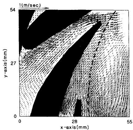
(a) Velocity Vectors
