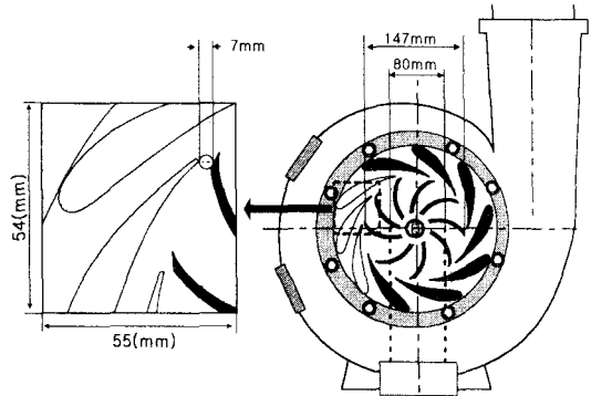
Fig.2 Definition of Measuring Region
