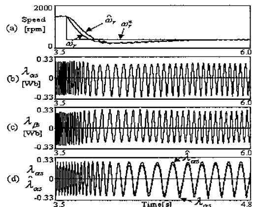
Fig. 4. Step response with LPF with fixed pole ( s = -1 ). (load torque : 6 [Nm], speed reference ( \omega_r^* ) : 1500 \rightarrow 400[rpm])
