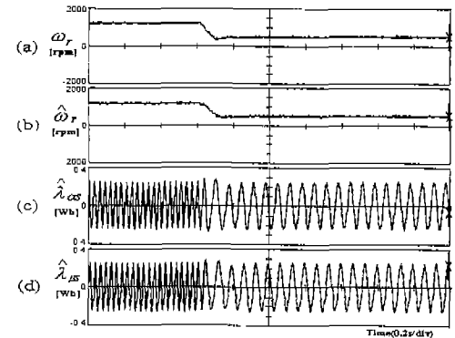
Fig. 8. Step response with programmable LPF. ( k=3 , load torque : 4[Nm], speed reference : 1000 \rightarrow 500[rpm])
