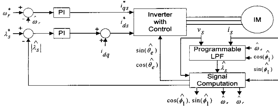
Fig. 3. Block diagram of speed sensorless stator flux orientation control drive.
