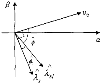
Fig. 1. Vector diagram of LPF and pure integrator.
