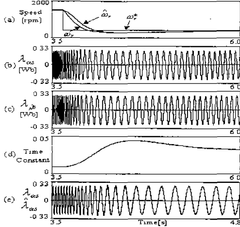
Fig. 5. Step response with programmable LPF. ( k=3 , load torque : 6[Nm], speed reference : 1500 \rightarrow 400[rpm])
