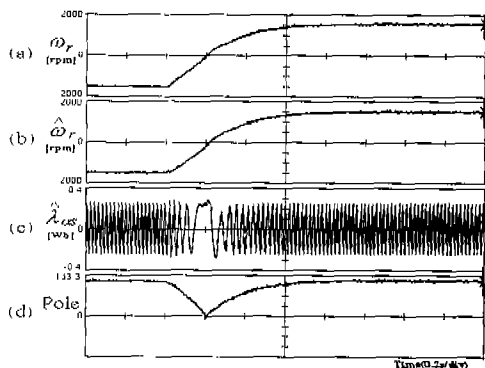
Fig. 10. Speed reversal operation with programmable LPF.( k=3 , no load, speed reference : -1500 \rightarrow 1500 [rpm])
