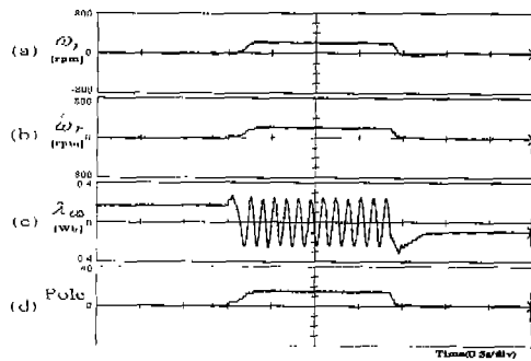
Fig. 9. Speed and flux waveforms with programmable LPF.( k=3 , no load, speed reference : 0 \rightarrow 200 \rightarrow 0 [rpm])
