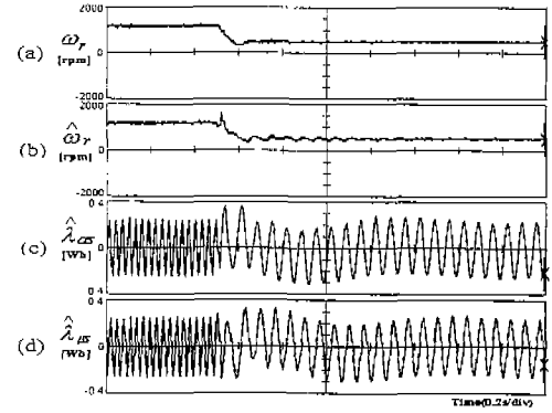
Fig. 7. Step response with LPF with fixed pole( s=-1 ). (load torque : 4[Nm], speed reference : 1000 \rightarrow 500[rpm])
