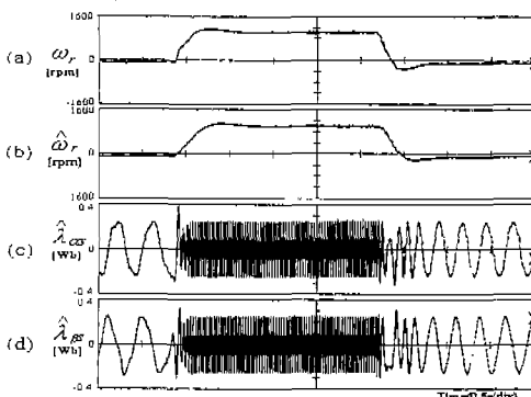
Fig. 6. Speed and flux waveforms with LPF with fixed pole( s=-20 ).(no load, speed reference : 0 \rightarrow 1000 \rightarrow 0[rpm])
