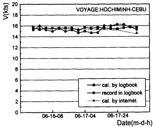
Fig. 6 Comparison of nominal speed loss
