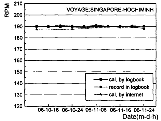
Fig. 5 Comparison of nominal RPM down
