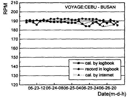
Fig. 9 Comparison of nominal RPM down
