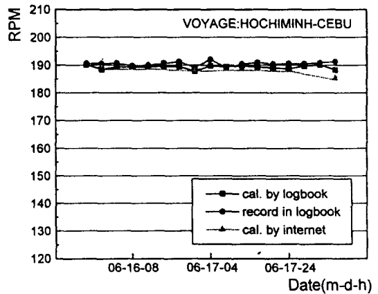
Fig.7 Comparison of nominal RPM down
