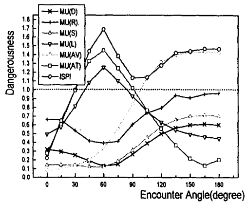
Fig.15 Dangerousness of seakeeping factors and ISPI at NBF 8
