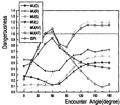
Fig.14 Dangerousness of seakeeping factors and ISPI at NBF 7
