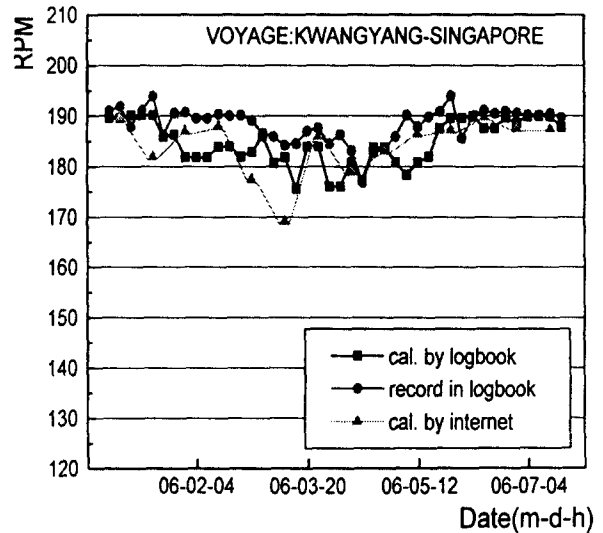
Fig. 3 Comparison of nominal RPM down
