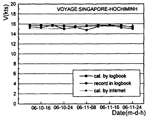
Fig. 4 Comparison of nominal speed loss
