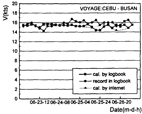
Fig. 8 Comparison of nominal speed loss
