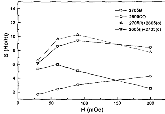
Fig. 1 The shielding effectiveness of 2705M & 2605CO as a cylinder shields in ac-field of 60 Hz.
