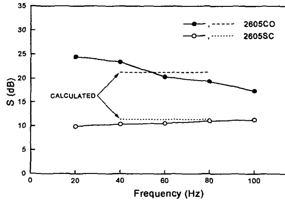
Fig. 2 The shielding effectiveness of 2605CO & 2605SC as a cylinder shields in 20~100 Hz.
