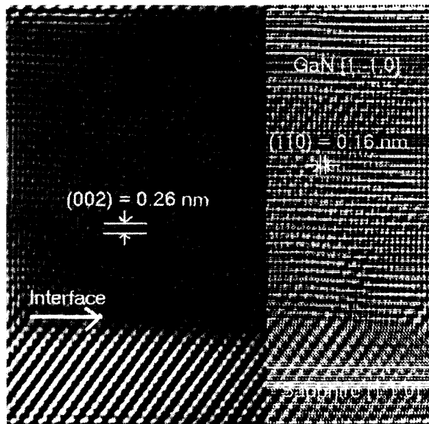
Figure. TEM lattice image of GaN thick film grown on sapphire(001).
