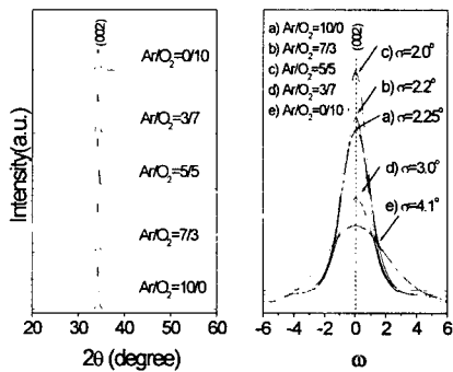
Fig. 2. The variation of \theta/2\theta and rocking curve spectra as a function of Ar/O 2 gas ratios at 100 w, 10 mT, 200°C
