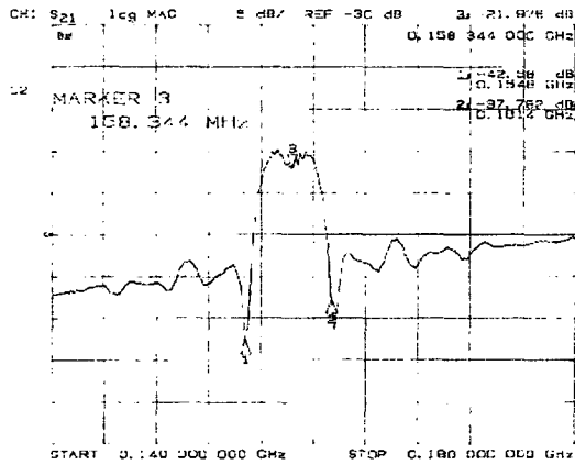
Fig. 5. Frequency response of ZnO SAW filter
