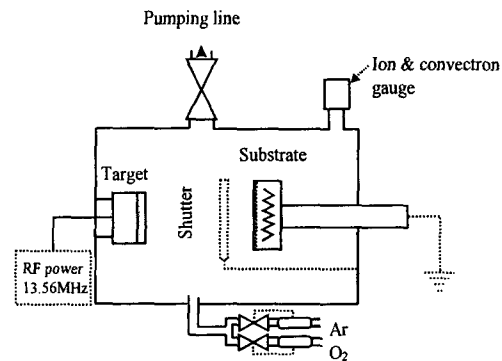
Fig. 1. Schematic diagram of R.F magnetron sputter system
