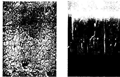
Fig. 3. SEM micrographs of ZnO films on glass as a function of Ar/O 2 =50/50 gas ratios at 100 w, 10 mT, 200°C
