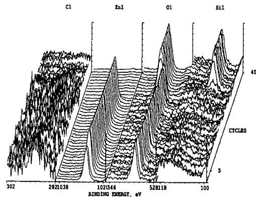
Fig. 4. XPS spectra of Zn1, O1, Si1 of ZnO films as a function of Ar/O 2 =50/50 gas ratios at 100 w, 10 mT, 200°C
