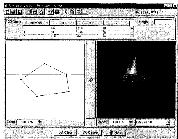
Fig. 6. Object Authoring Tool
