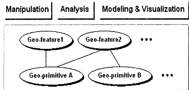
Fig. 2. Geo-features and geo-primitives designed for the efficiency of manipulation, analysis, modeling and visualization of 3D geographic information.
