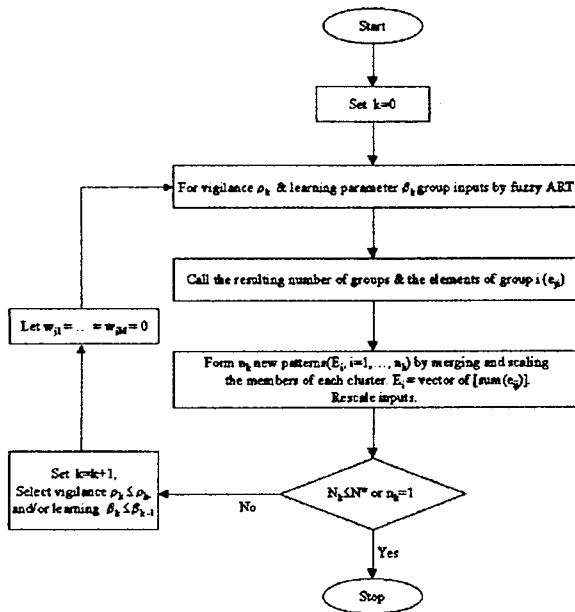
Fig 2. Modified Fuzzy ART Neural Network
