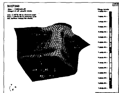
Fig. 4 The effective strain distribution at the BHF, 260N
