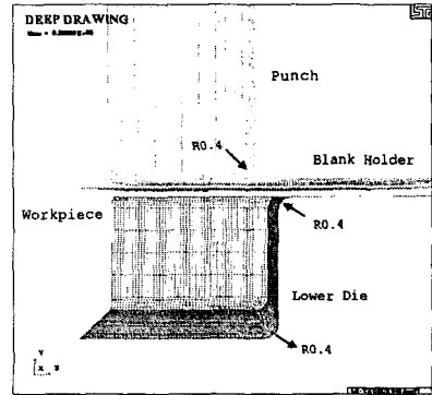
Fig. 3 The FE-model for rectangular cup drawing
