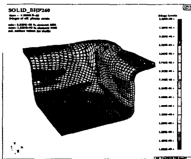
Fig. 6 The effective strain distribution of the brick element type
