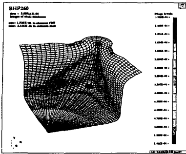
Fig 5 The thickness distribution at the BHP, 260N
