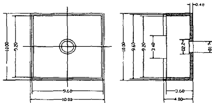
Fig. 2 The final product geometry(unit:mm)
