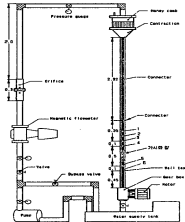
Fig. 1 Schematic diagram of experimental apparatus ; all dimensions in m
