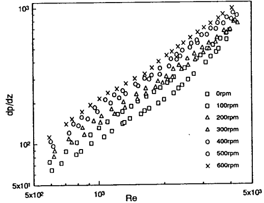
Fig. 3 Total dp/dz of glycerine-water solution as a function of Re at 0~600rpm
