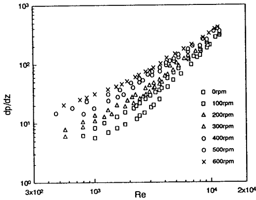
Fig. 2 Total dp/dz of water as a function of Re at 0~600rpm
