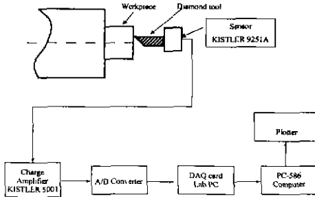
Fig. 8 Experimental setup
