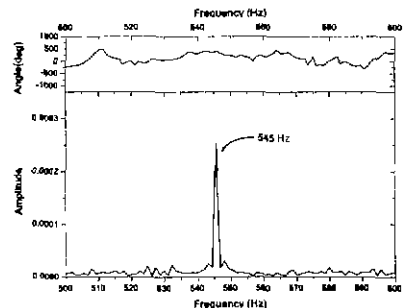
Fig. 7 Frequency spectrum for tool holder on DTM in the z-direction
