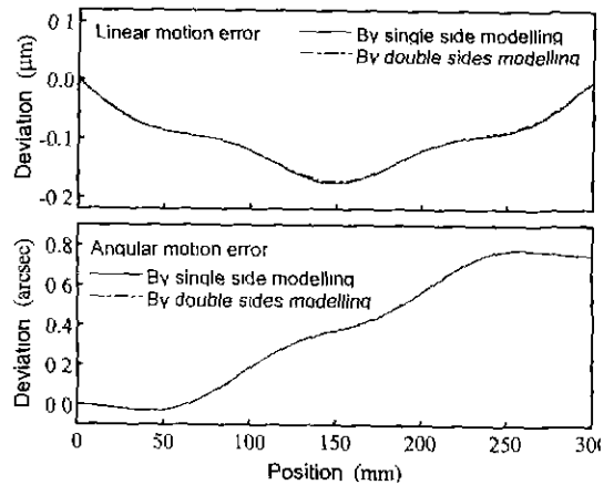
Fig. 5 Comparison of motion accuracies by two analysis methods(against 1 and 5 period of rail profile)
