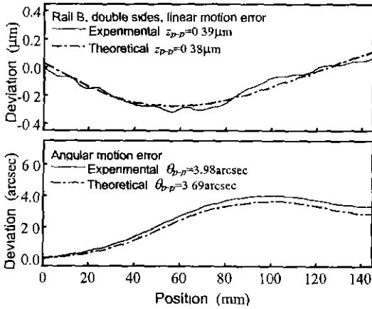
Fig. 10 Motion errors of double sides table against rail B
