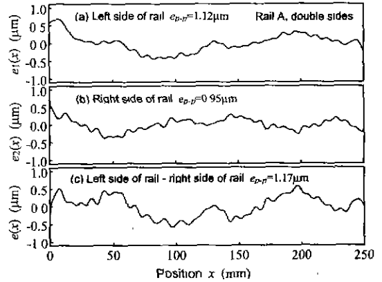
Fig. 7 Form errors of rail A
