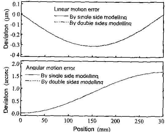
Fig. 4 Comparison of motion accuracies by two analysis methods(against 1 period of rail profile)
