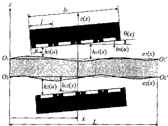
Fig. 1 Analysis model of double-sides hydrostatic table
