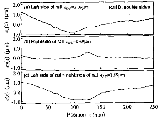
Fig. 8 Form errors of rail B
