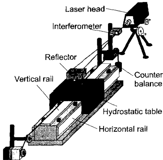
Fig. 6 Schematic diagram of experimental setup
