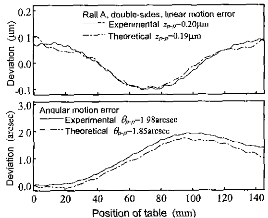
Fig. 9 Motion errors of double sides table against rail A
