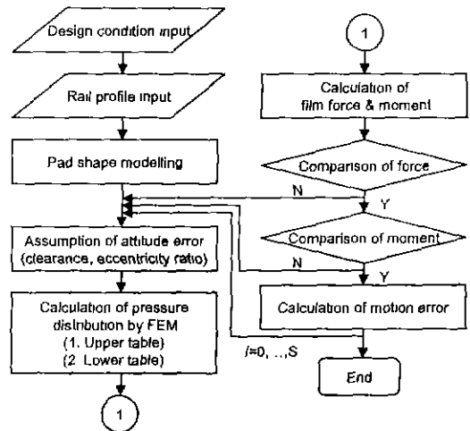
Fig. 2 Algorithm for calculating the motion error of double sides table
