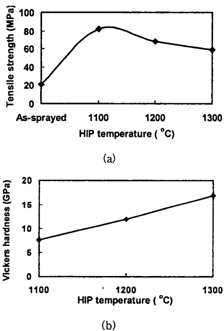
Fig. 2. Variations of Vickers hardness (b) and tensile strength (a) of \text{Al}_2\text{O}_3 coating HIPed at various temperature
