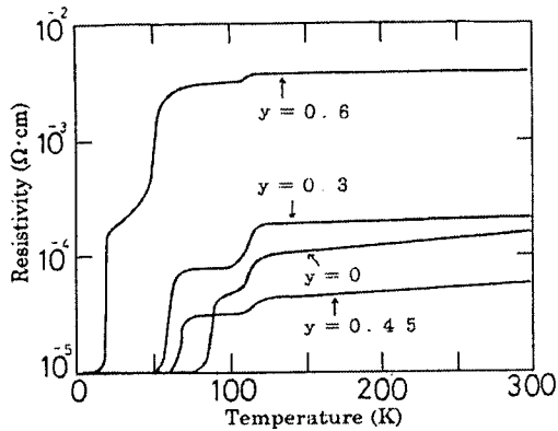
Fig.5 Temperature dependence of resistivity for \text{Bi}_{1-y}\text{P}_y\text{SrCaCu}_2\text{O}_x ( M=\text{Sb, As, P} )
