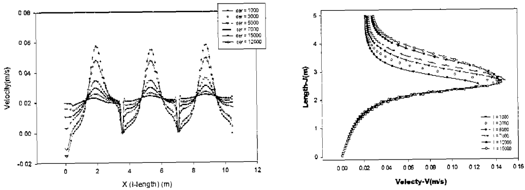
그림5. V-velocity convergence test with iteration at sedimentation basin inlet zone(j=45) & 2nd inlet channel (50,j)
