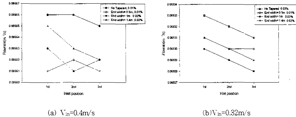
그림7. Flow rate calculation with V_{inlet} & tapered type(channel width; 2.4m)
