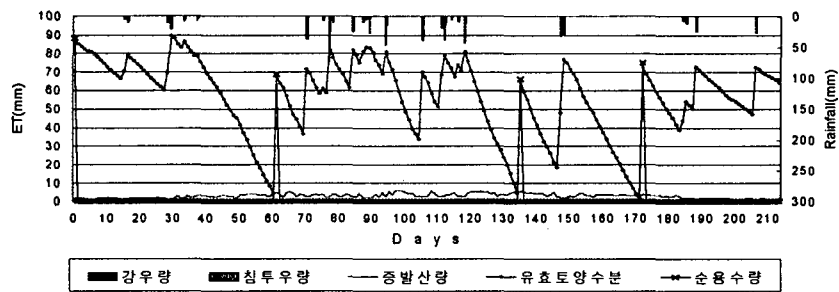
Fig. 4.6 Crop evapotranspiration and water consumption (Apple)
