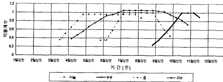
Fig. 4.1 Crop coefficient
