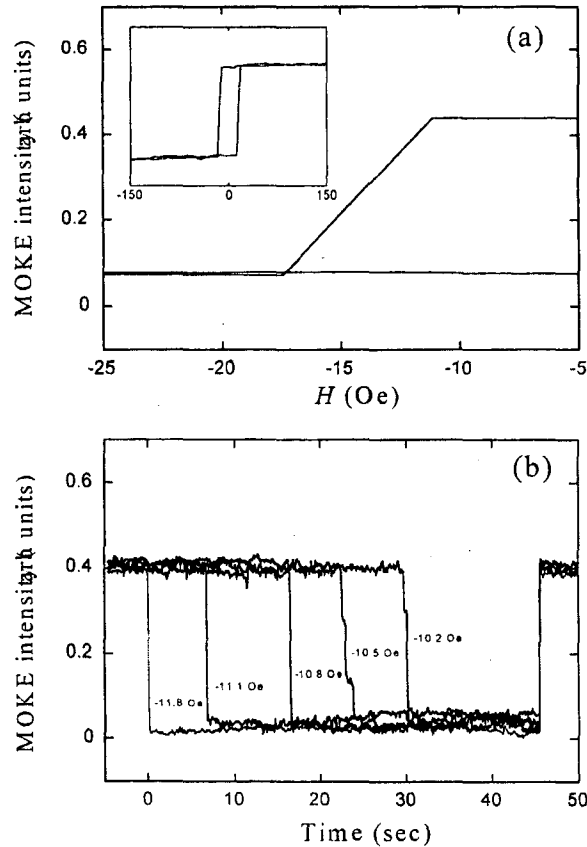
Fig. 4 (a) Part of a MOKE loop measured at a sweep rate of 0.01 kOe/sec and (b) magnetic relaxation curves of 55 Å Fe/GaAs(001) film under a constant reverse field. The inset of (a) shows the sharpness of the loop at low sweep rate. For time t < 0 and t > 45 seconds the sample was saturated in the positive direction.
