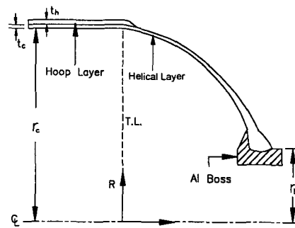
Fig 1. Cross-section of filament wound pressure tank
