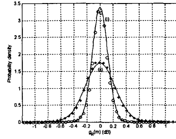
Fig. 3 Distribution of g_R(m) in typical fixed wireless channel: (i) f_d T_F = 0.0108 , (ii) f_d T_F = 0.0216
