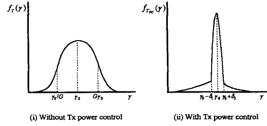
Fig. 2 SNR distribution of the received signal in fixed wireless channel
