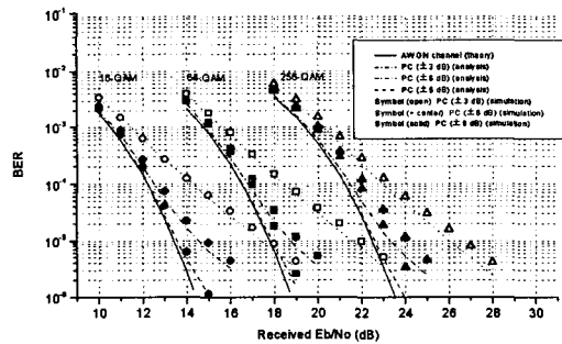
Fig. 7 BER performance of the proposed QAM transceiver in typical fixed wireless channel with flat fading
