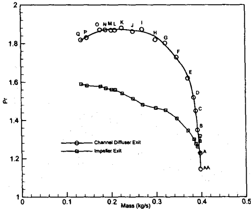
Fig. 5 Performance map of compressor
