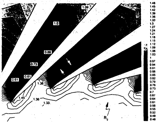
(a) Static pressure contour in flow condition AA.
