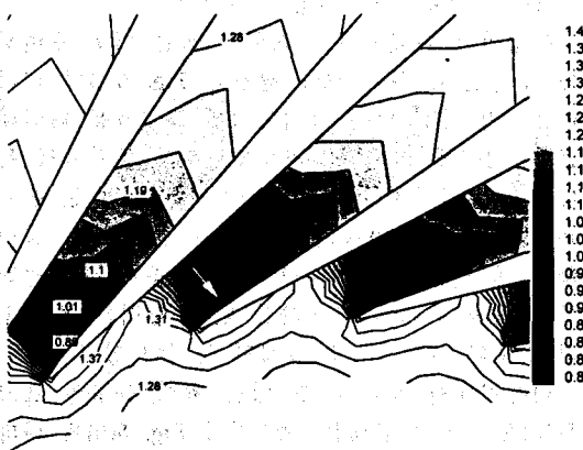
(c) Static pressure contour in flow condition B.
