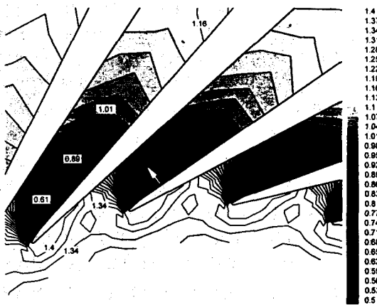
(b) Static pressure contour in flow condition A.
