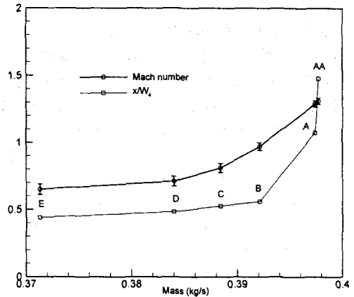
Fig. 7 Location and estimated Mach number at the minimum pressure location in channel.
