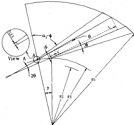
Fig. 2 Configuration of channel diffuser
