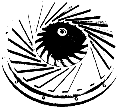
Fig. 1 Test impeller and channel diffuser
