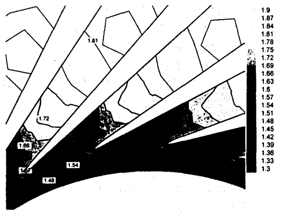
(e) Static pressure contour in flow condition I.
