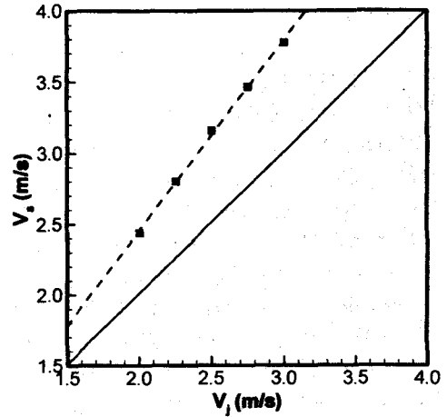
Fig. 7 Effect of the jet velocity on the mean sheet velocity for D_j=1.0 mm, \theta=60^\circ . The solid line represents the mean sheet velocity( V_s ) equals the jet velocity( V_j ).
