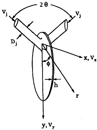
Fig. 1 A liquid sheet formed by two impinging jets
