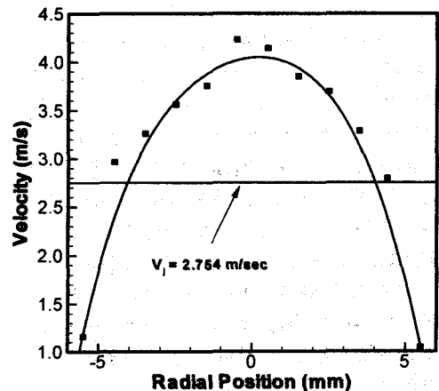
Fig. 3 Velocity distribution at the cross-section of the jet for D_j=1.0 mm, V_j=2.75 m/s.
