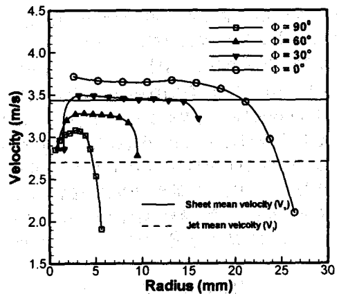
Fig. 5 Distribution of the sheet velocity for D_j=1.0 mm, \theta=60^\circ , V_j=2.7 m/s.
