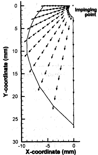
Fig. 4 Distribution of the sheet velocity vector on the overall liquid sheet for D_j=1.0 mm, \theta=60^\circ , V_j=2.7 m/s.
