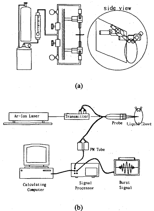
Fig. 2 Schematic diagram of the experimental apparatus; (a) impinging jet system, (b) LDV system
