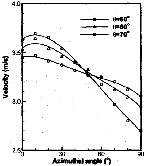
Fig. 6 Effect of the impinging angle on the sheet velocity for D_j=1.0 mm, V_j=2.7 m/s.
