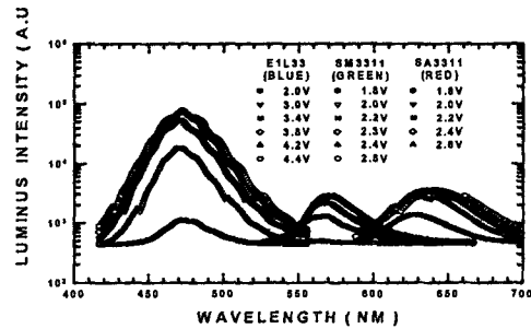
Fig. 2. Spectral power distribution of LEDs.
