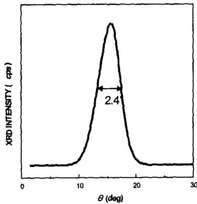
Fig 5. Rocking curve deposited at Ramp method ZnO thin films
