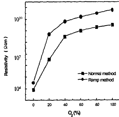
Fig 6. Compare Ramp method with Normal method of Resistivity
