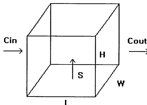
<Fig2> Box Model
