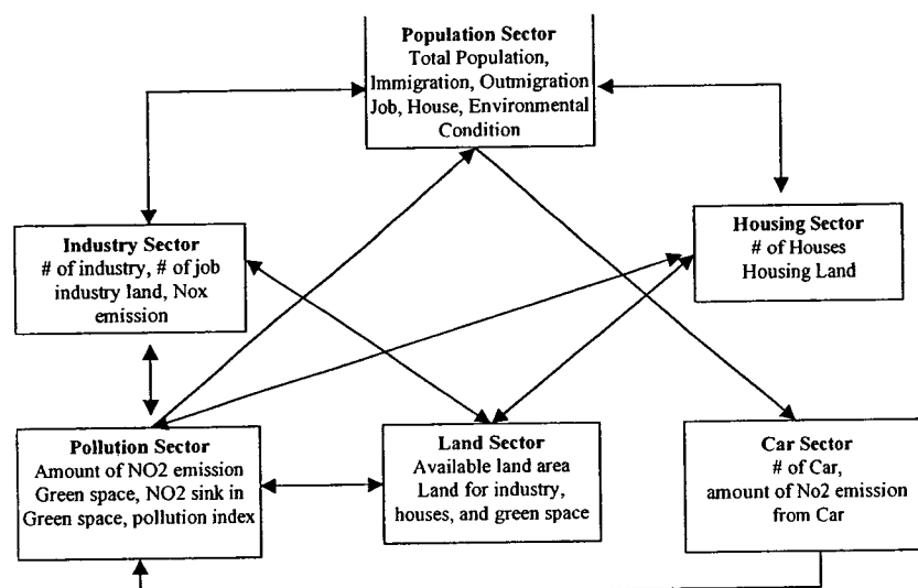
<Fig.1> Environmental Carrying Capacity Conceptual Model
