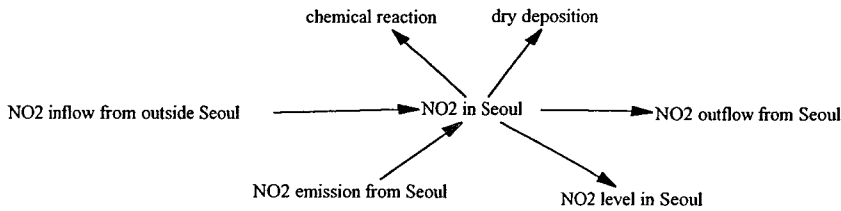
<Fig3> Box Model and Causal Loop
