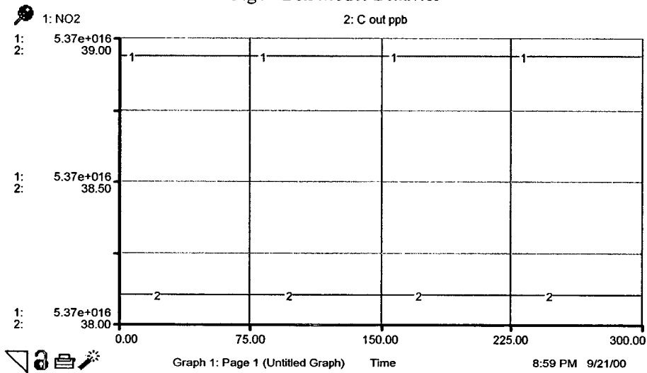
<Fig4> Box Model Behavior
