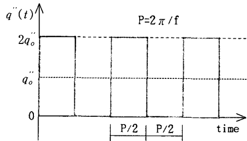
Fig. 2 Time-periodic heat flux imposed on one sidewall.
