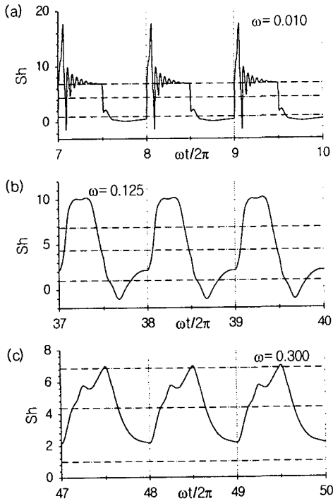
Fig. 5 Temporal behavior of Sh(t) . The three horizontal lines in the frames indicate the values of Sh_s for \gamma=0 , \gamma=2 , and \gamma=4 .
