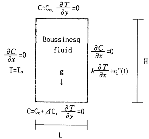
Fig. 1 Sketch of the flow configuration.
