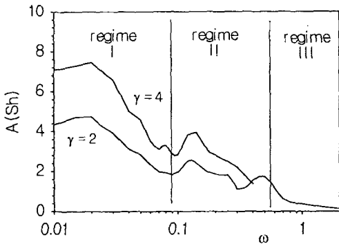
Fig. 4 Variation of A(Sh) vs. \omega .
