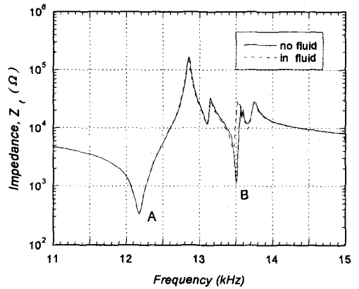
Fig. 5 Impedance curve of the transducer-rod system measured as a function of the frequency.
