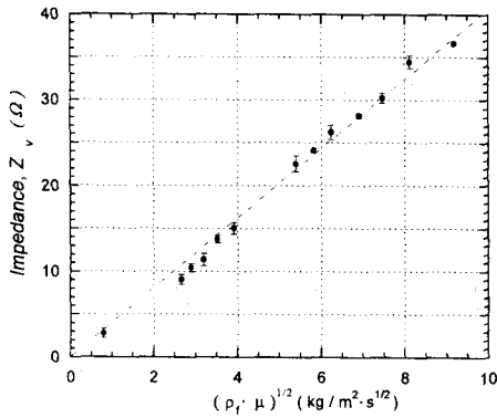
Fig. 6 Electrical impedance measured at the frequency \omega_\theta = 2\pi \times (12.1 \times 10^3 \text{ Hz}) and depicted as a function of (\rho_f \cdot \mu)^{1/2} .
