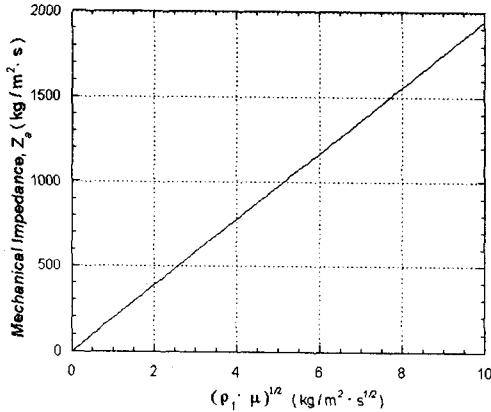
Fig. 3 Mechanical impedance calculated for the frequency \omega_\theta = 2\pi \times (12.1 \times 10^3 \text{ Hz}) and depicted as a function of (\rho_f \cdot \mu)^{1/2} .
