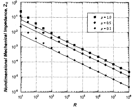
Fig. 2 Nondimensional mechanical impedances obtained from the exact (symbols) and approximate (solid lines) solutions.
