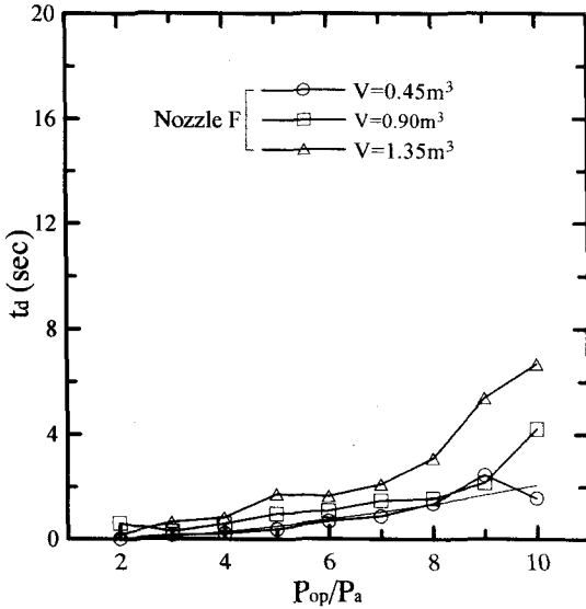
(c) Nozzle F
