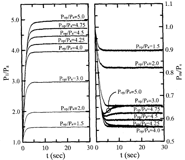
Fig. 5 P_1/P_a and P_{os}/P_a vs t
