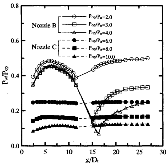
Fig. 3 Static pressure distributions along the wall surface
