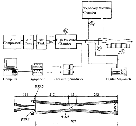
Fig. 1 Experimental facility and ejector dimension
