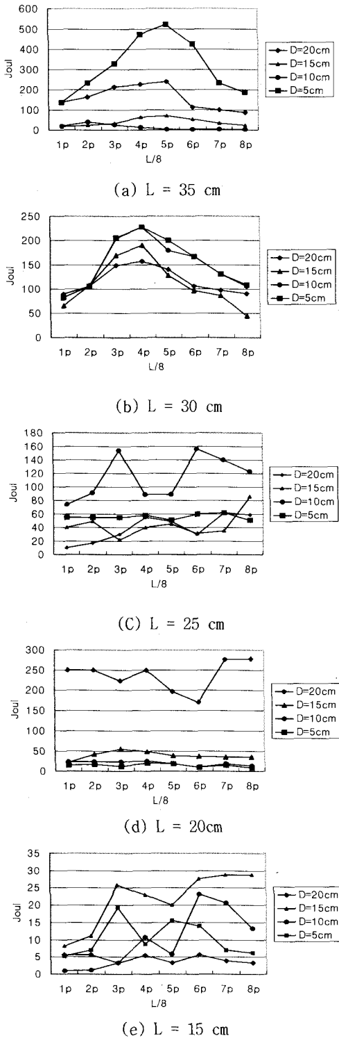
Fig. 2 Heat energy distribution with different aspect ratios of the modelled fire clay.
