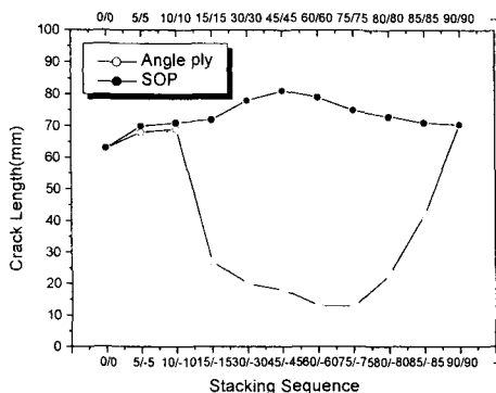
Fig. 13 Crack length for angle ply and SOP FML
