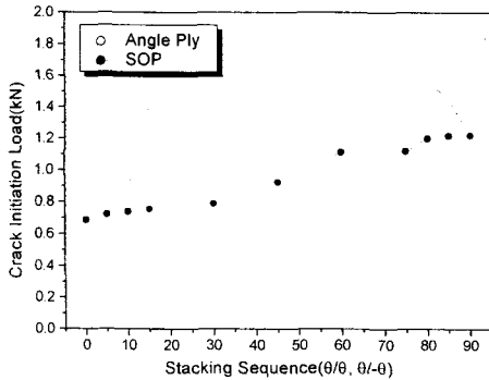
Fig. 12 Crack initiation load for angle ply and SOP FML
