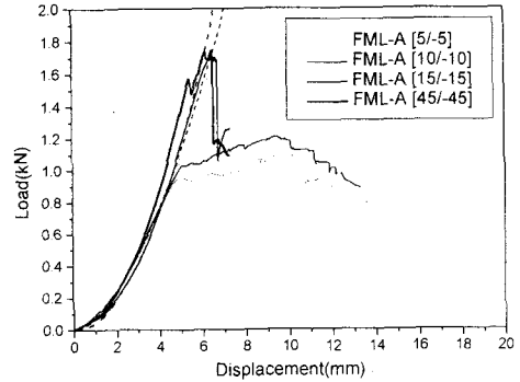
Fig. 8 Indentation curve of angle ply FML
