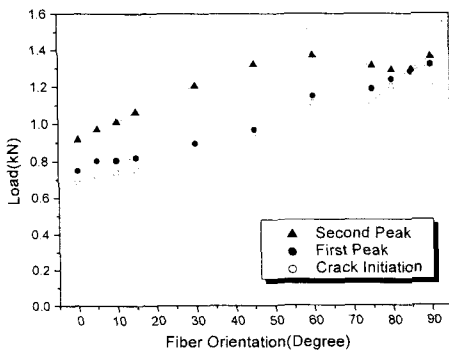
Fig. 7 Behavior of crack initiation, first and second peak varied with fiber orientation
