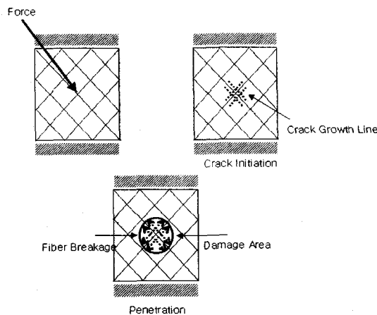
Fig. 10 Schematic diagram of damage process of angle ply FML with high fiber orientation
