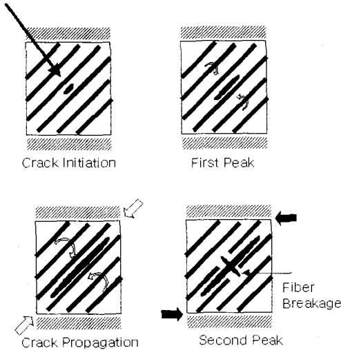
Fig. 6 Schematic diagram of damage process of SOP FML with high fiber orientation
