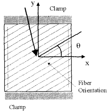
Fig. 2 Boundary conditions and fiber orientation
