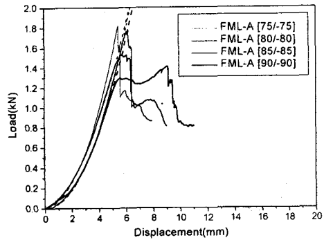
Fig. 11 Indentation curve of angle ply FML
