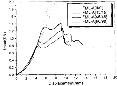
Fig. 5 Indentation curve of SOP FML
