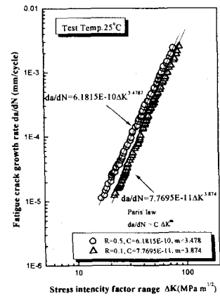
Fig.3 Relation between stress intensity factor range and fatigue crack growth rate at 25℃
