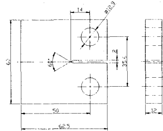
Fig. 1 Geometry and configuration of compact tension specimen
