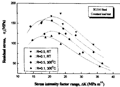
Fig.7 Relation between the residual stress on fracture surface and stress intensity factor range
