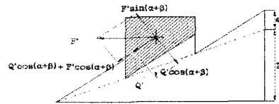
Fig. 4 Load on stairs type screw threads (when unscrewing)
