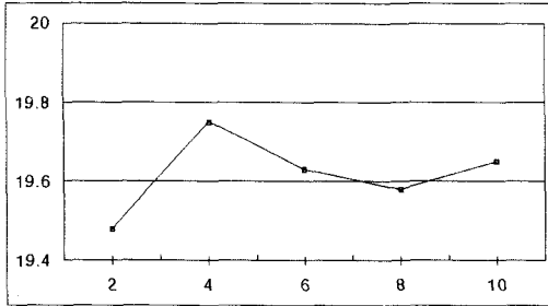
Fig. 18 Maximum equivalent stress according to rotation angle
