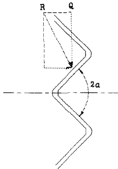
Fig. 3 Sectional plan of a triangular screw
