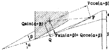
Fig. 2 Load on stairs type screw threads (when screwing)
