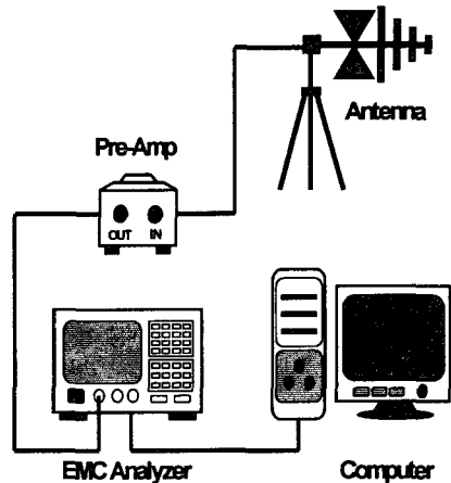
Fig. 2.2 HFPD measurement system.
