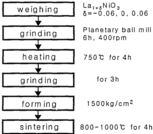
Fig. 1. Proecessing of LaNiO 3 ceramics.
