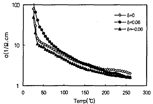
Fig. 7. Temperature dependence of conductivity \text{La}_{1-x}\text{NiO}_3 ceramics.
