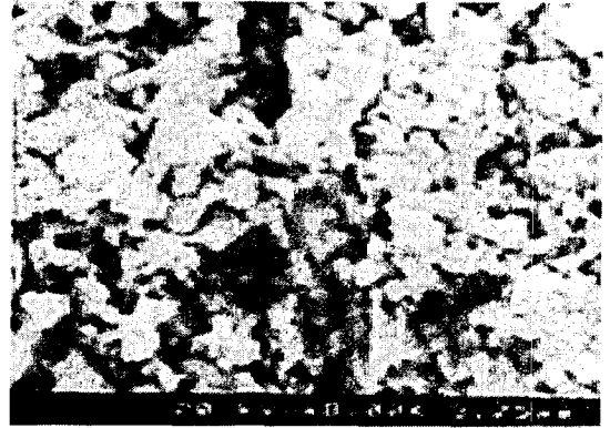
Fig. 5. Scanning electron micrograph of \text{La}_{1-x}\text{NiO}_3 ( \delta = 0 ) sintered at 900°C
