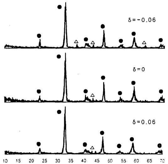
Fig. 2. XRD traces of La 1+ \delta NiO 3 sintered at 900℃ ( \delta = -0.06, 0, 0.06 ). (●:LaNiO 3 , \Delta :NiO)
