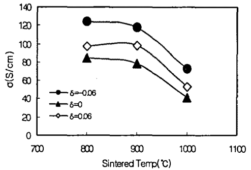
Fig. 6. Electrical conductivity ( \sigma ) of \text{La}_{1-x}\text{NiO}_3 ceramics as a function of temperature.
