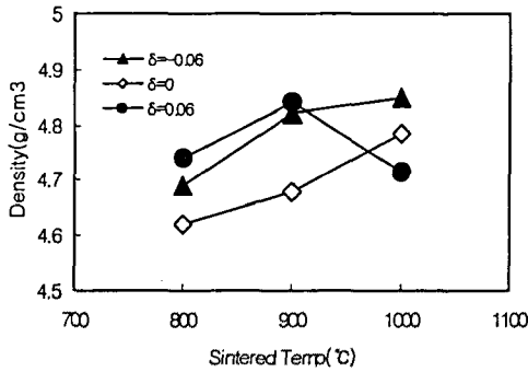
Fig. 4. Density of \text{La}_{1-x}\text{NiO}_3 ceramics as a function of temperature.
