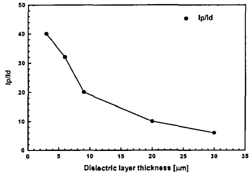
Fig 5. I_p/I_d plot as a function of Dielectric layer thickness
